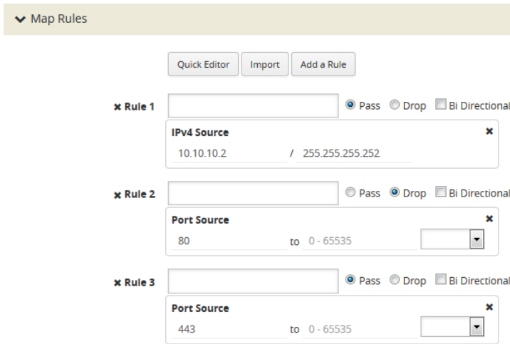
Figure 47 Rules Added with the Quick Rule Editor
