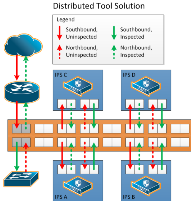
Figure 76 Multiple Tool Arrangement
