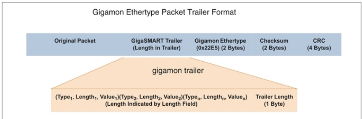
Figure 173 GigaSMART Trailer Format
