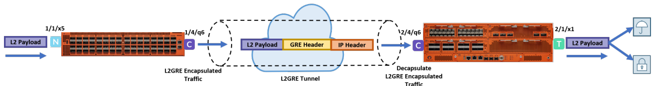
Figure 31 L2GRE Tunnel Encapsulation and Decapsulation
