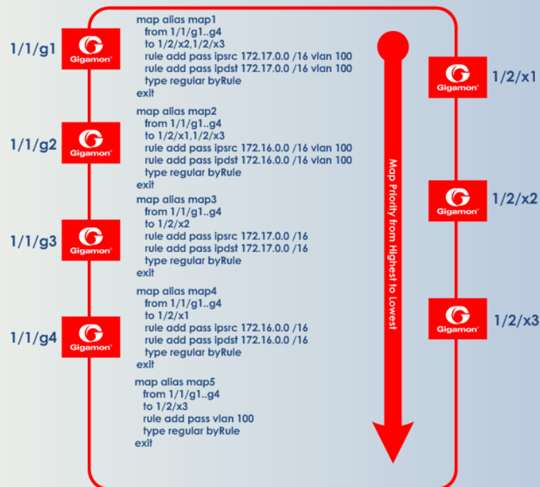
Figure 45 Sending Subnets and VLANs to Different Ports
