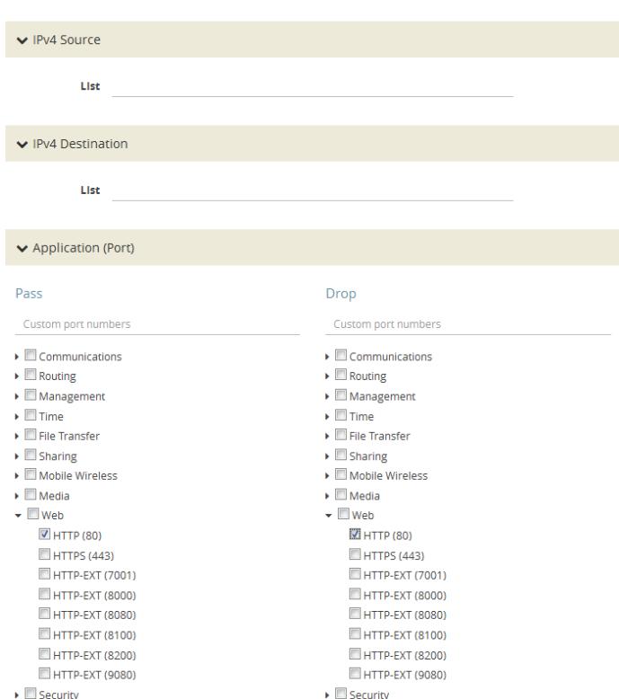
Figure 46 Custom Port Number Selected in Quick Rule Editor
