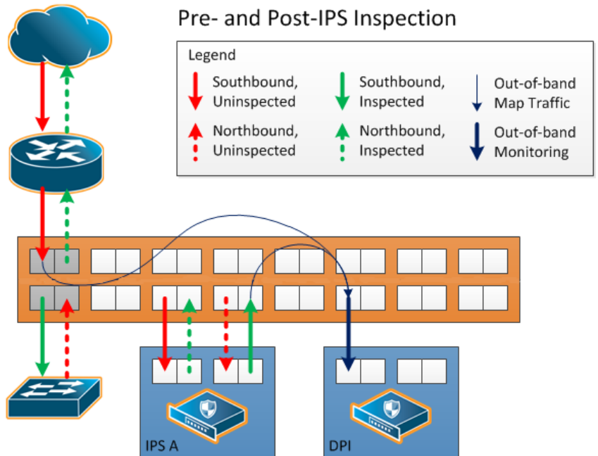
Figure 80 Out-of-Band Arrangement
