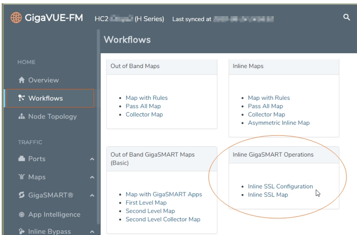
Figure 108 Select Inline SSL Map Configuration
