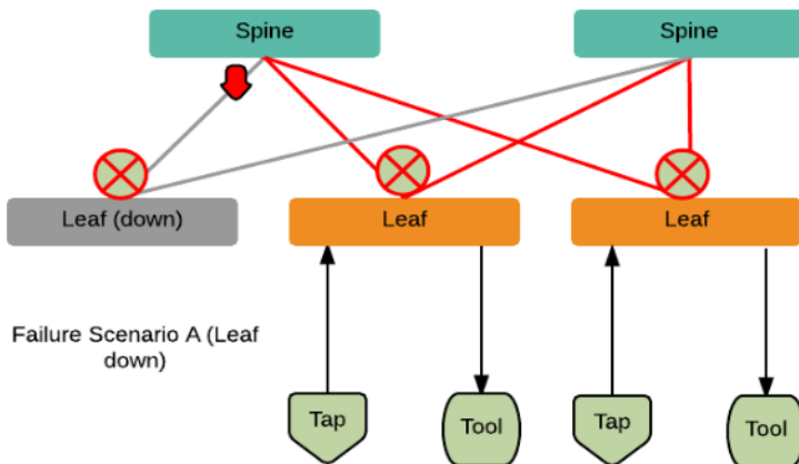
Figure 30 Leaf Node Failure
