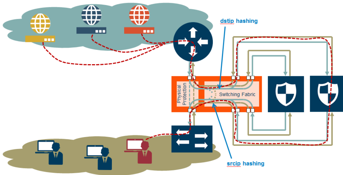
Figure 95 Asymmetrical Hashing
