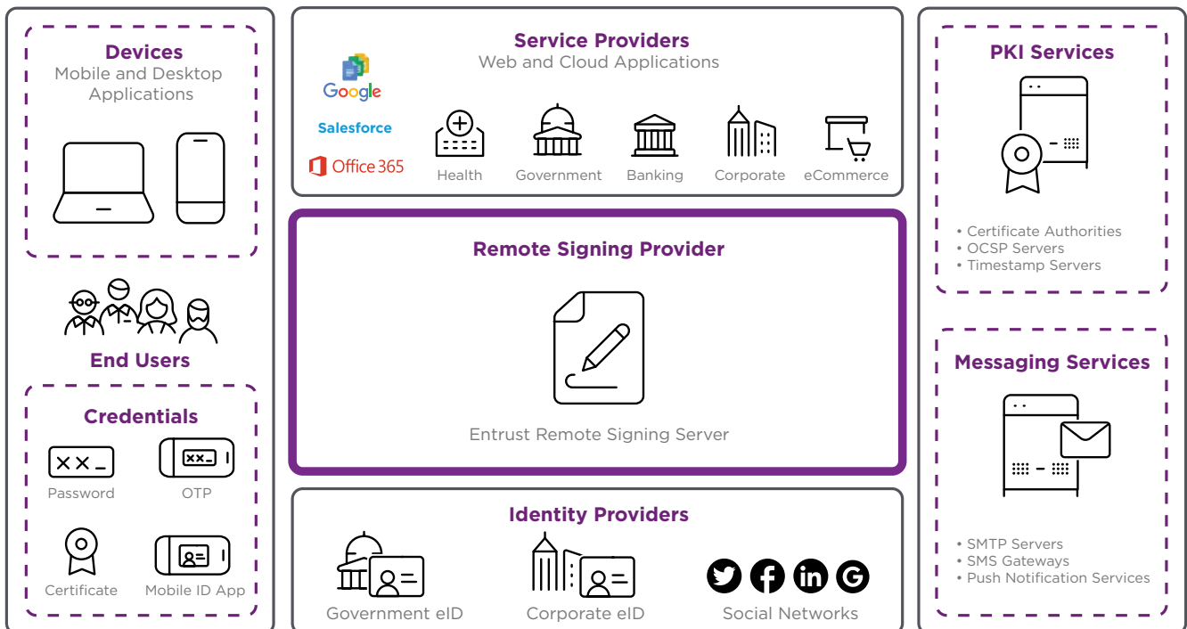
Figure 2. Relationship of the TrustedX eIDAS Platform with other systems
