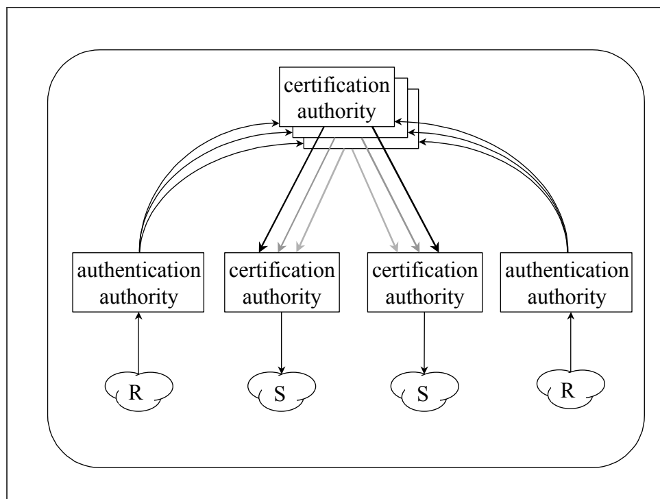
Figure 15 – Two-tier hierarchy
