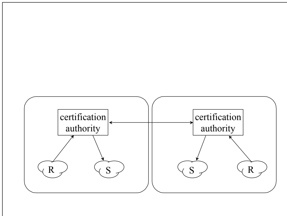
Figure 14 – Direct cross-certification
