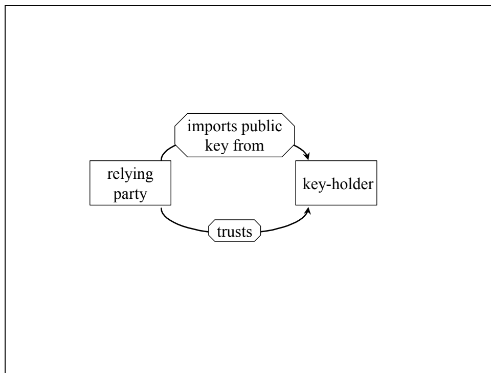
Figure 1 – Entity Relationship
