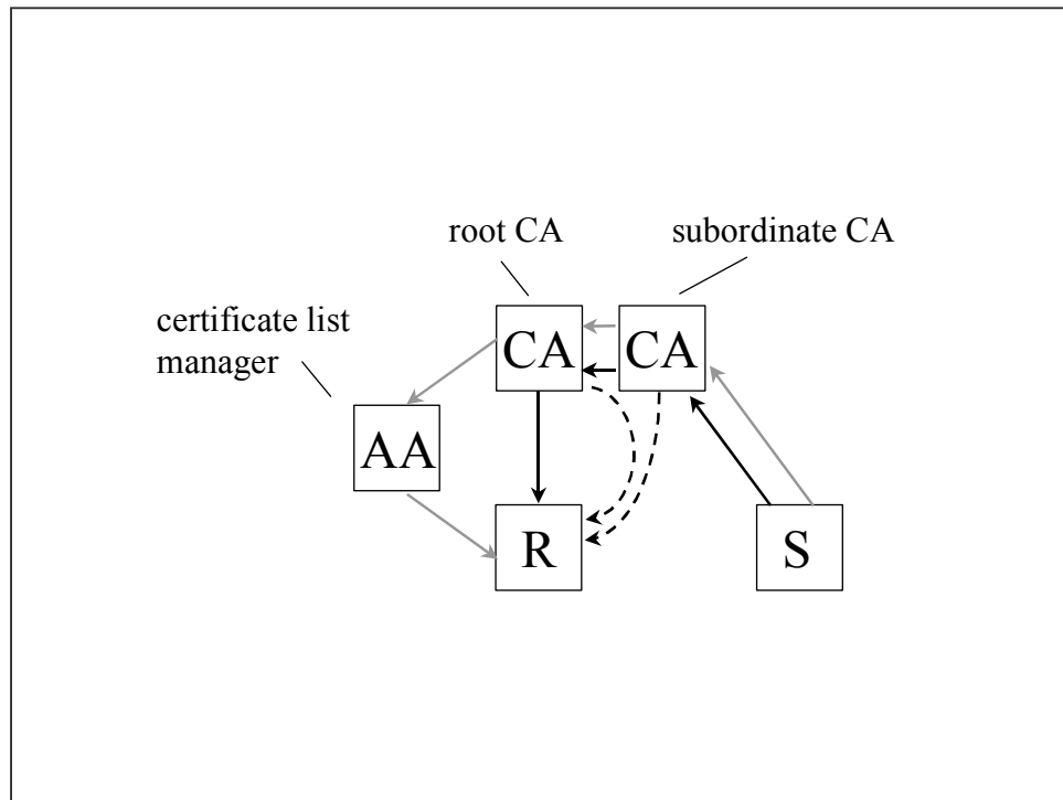
Figure 10 – Two-tier hierarchy
